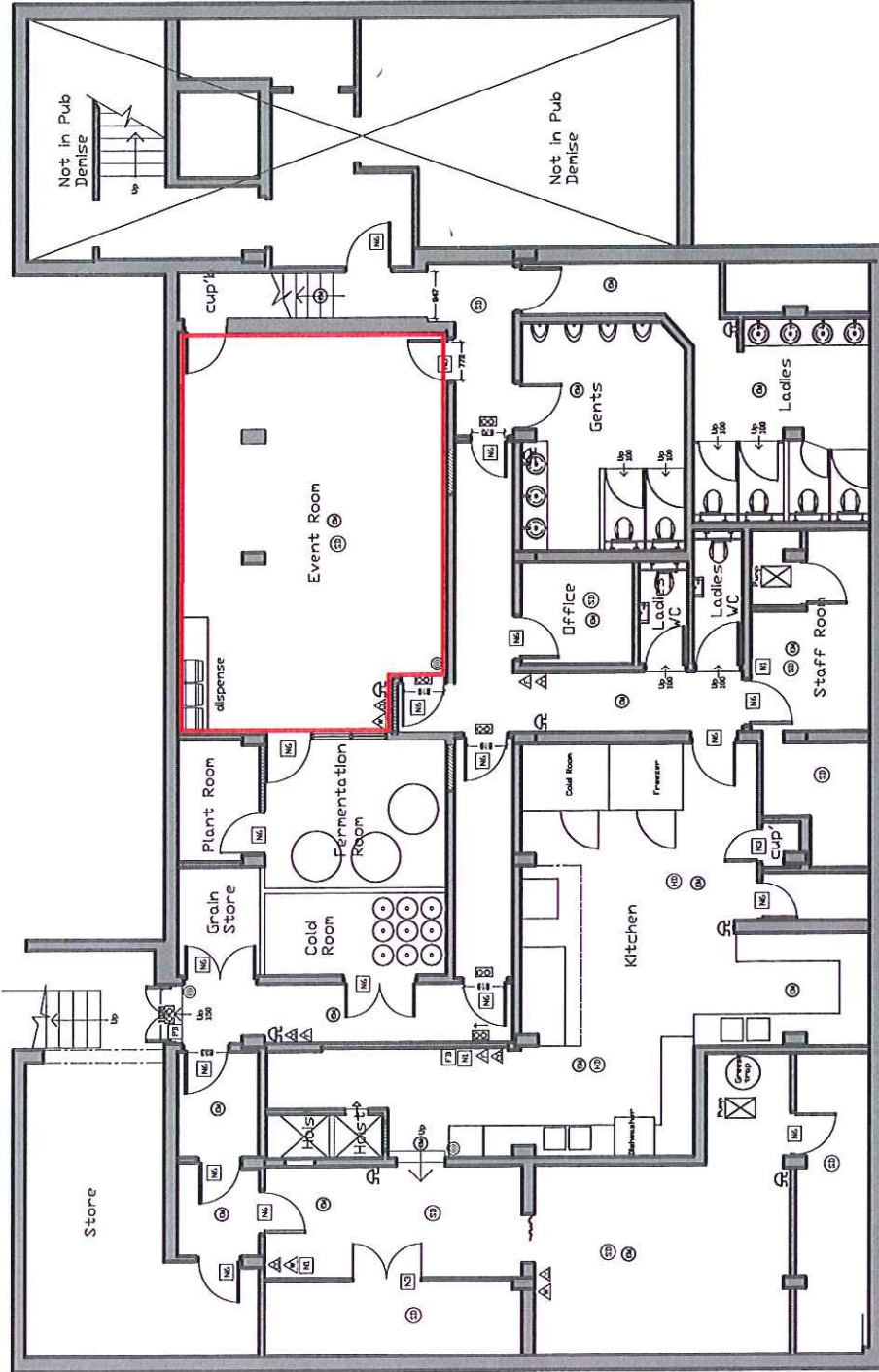
BASEMENT LAYOUT PLAN
